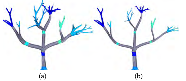
Fig. 9. Given an arbitrary tree-model (a), we apply allometry rules to further refining its branching structure (b).
